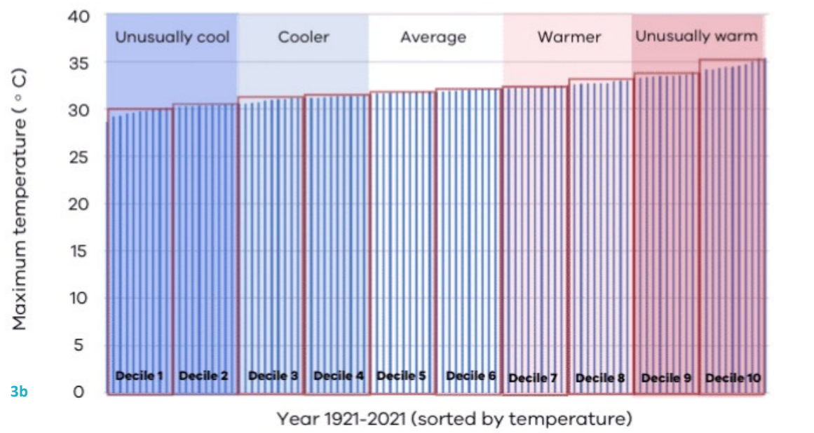
Figures 3a and 3b. Decile bar graphs showing August – October rainfall for 146 years (3a at top) and December – February maximum temperatures for 101 years (3b) in Dubbo, NSW. Reproduced from Agriculture Victoria’s eLearning course ‘Using seasonal climate prediction tools’.
