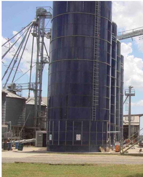
Photograph 5 – Typical reconstitution silos
