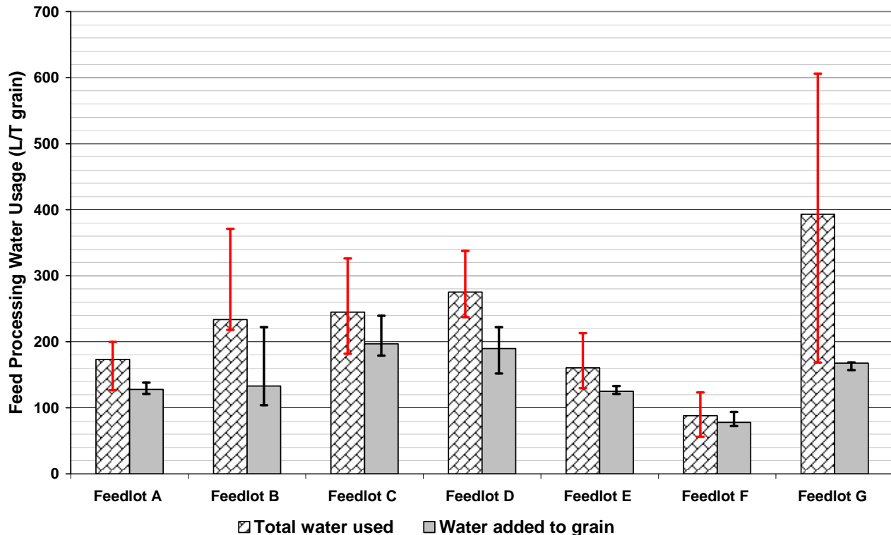
Figure 47 – Total feed processing water usage (L/t grain)
