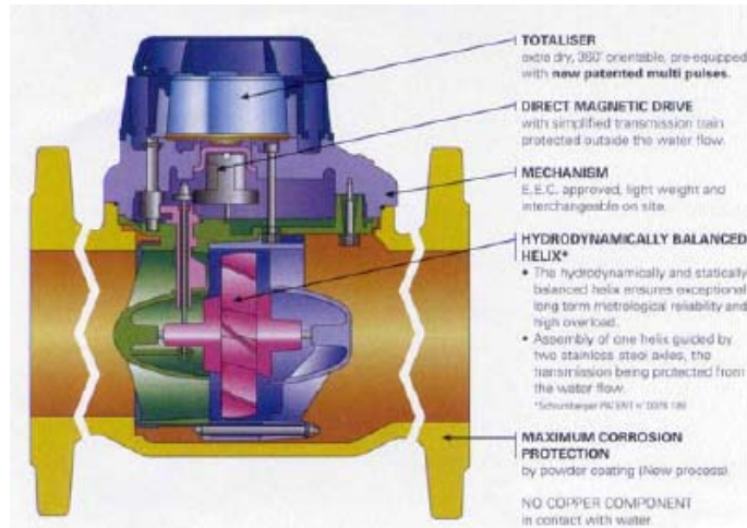
Photograph 20 – ManuFlo SW Turbine type water meter
