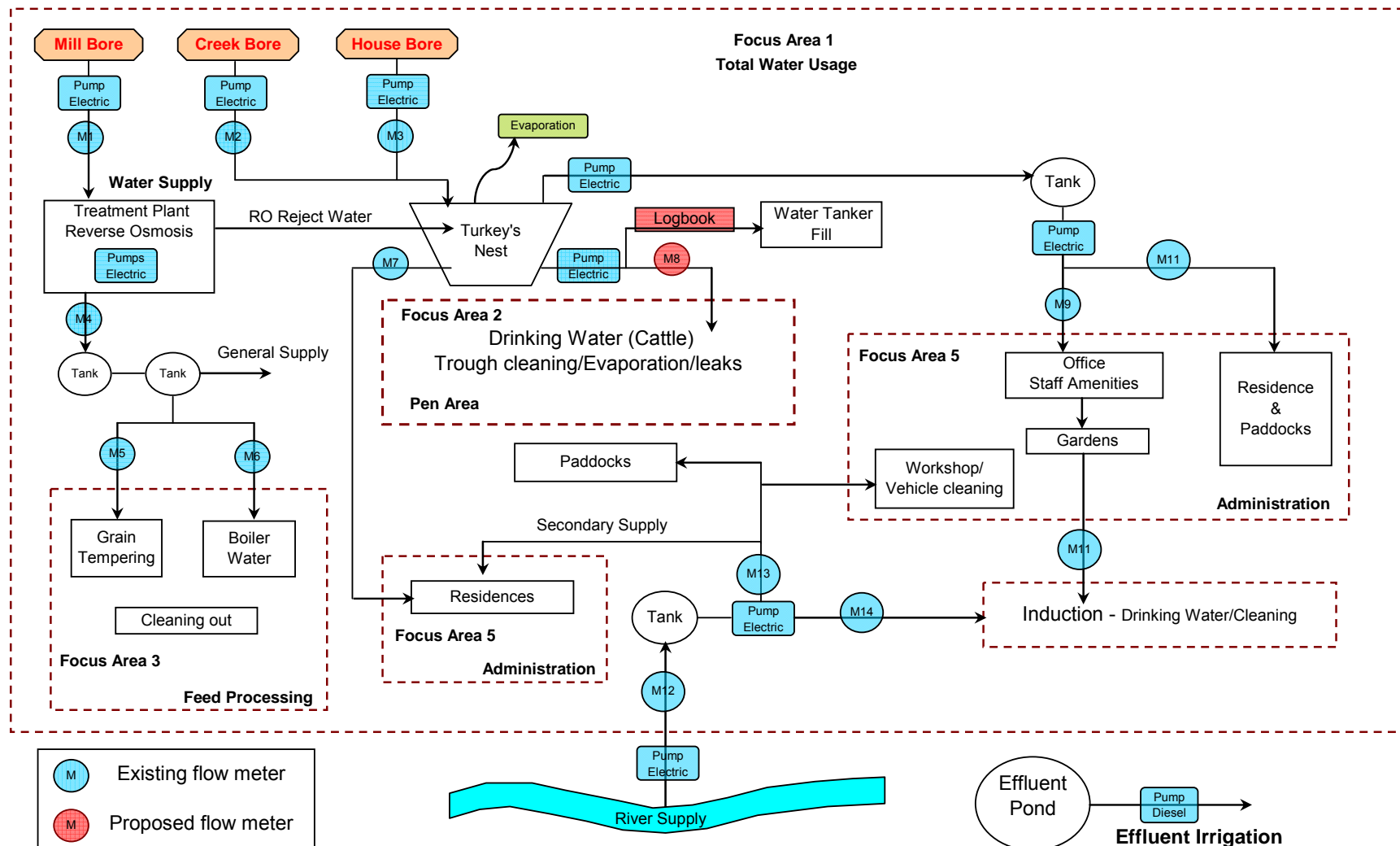
Figure 13 – Water system reticulation layout – Feedlot G
