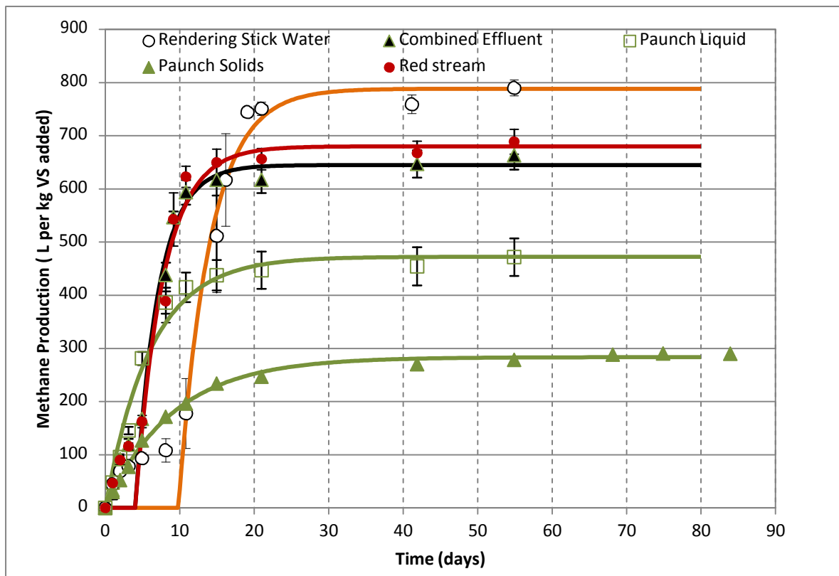
Figure 8 Results from biochemical methane potential (BMP) tests of select sample locations at Site E. Error bars indicate 95% confidence errors from triplicate batches. The line indicates the model used to return key parameters.
