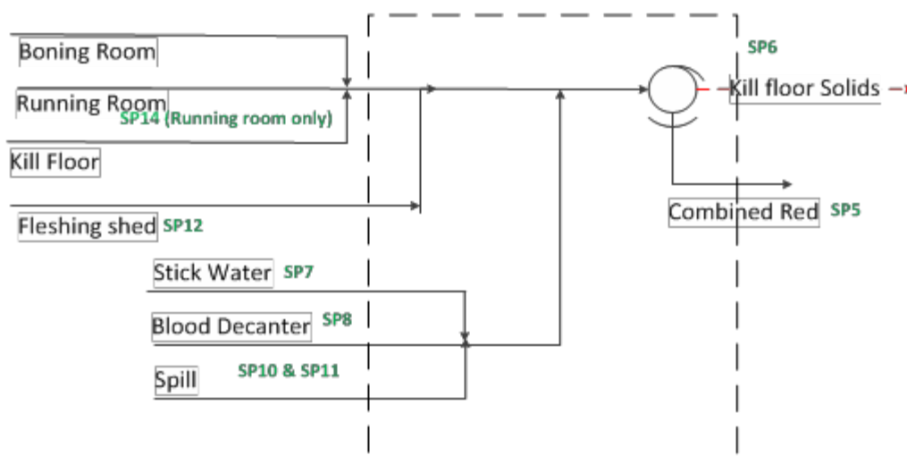
Figure 10 Flowsheet used for mass balance around red wastewater streams (SP7, SP8, SP10, SP11, SP12 and SP14 were considered feed streams; SP5 and SP6 were considered the mixed effluent).
