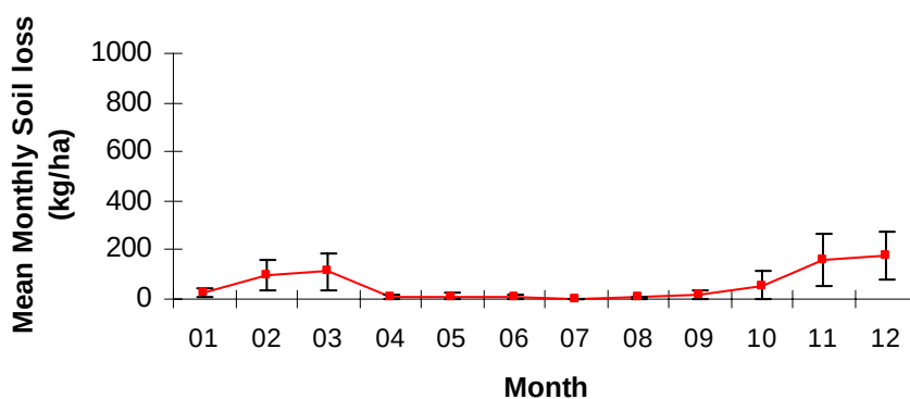
Figure 9.31 Mean monthly soil loss (kg/ha) averaged over all plots and four years at the poplar box site.
