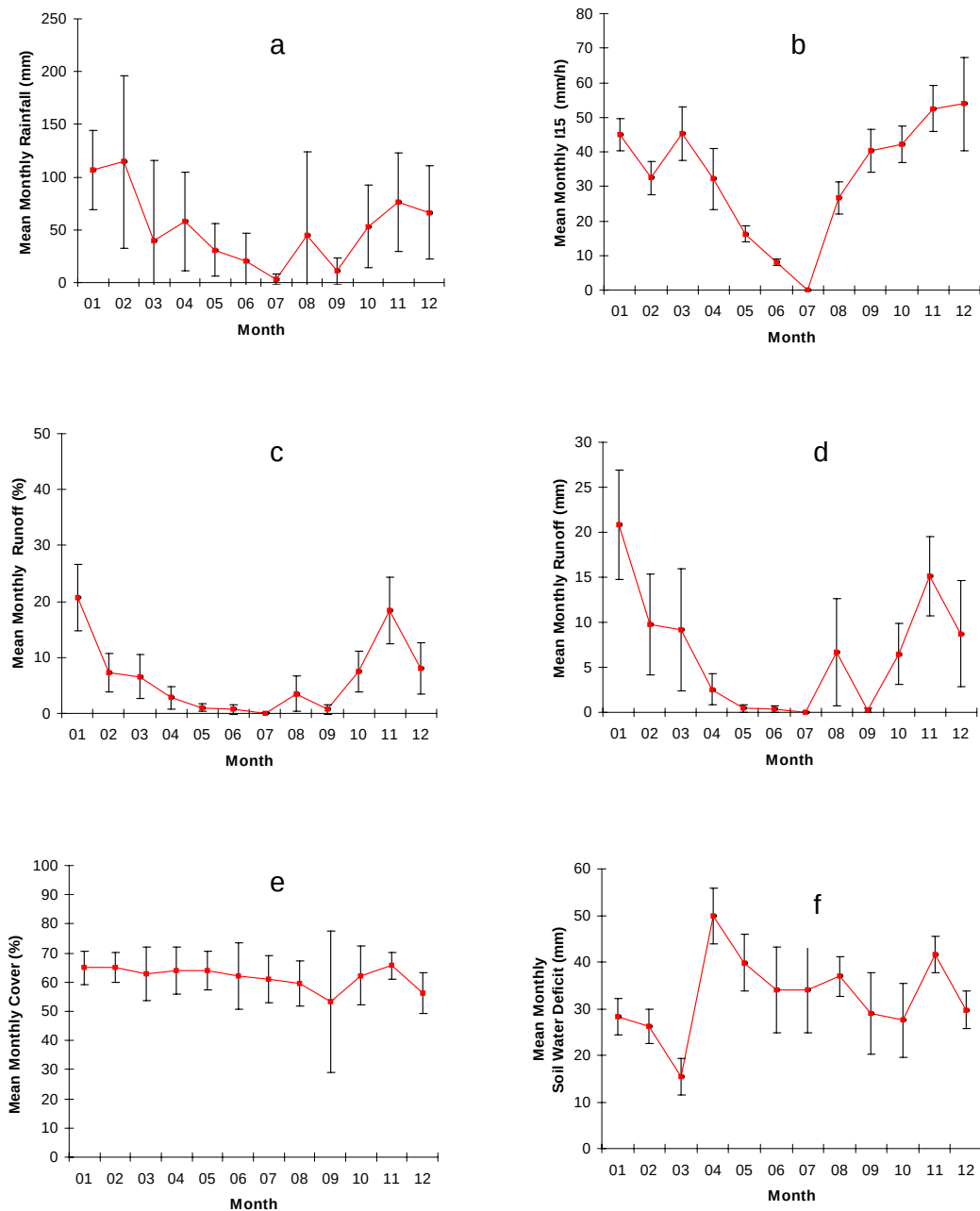
Figure 9.7 Mean Monthly (a) rainfall (mm), (b) I_{15} intensity (mm/h), (c) runoff (% of rainfall) (d) runoff (mm), (e) ground cover (%) and (f) soil water deficit (mm), averaged over all plots and five years at the ironbark site. [ Bars on data points show the Standard Deviation of the value plotted. ]
