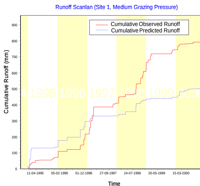
Figure 11.5 Poor fit between measured runoff and Scanlan model predictions at the ironbark site.
