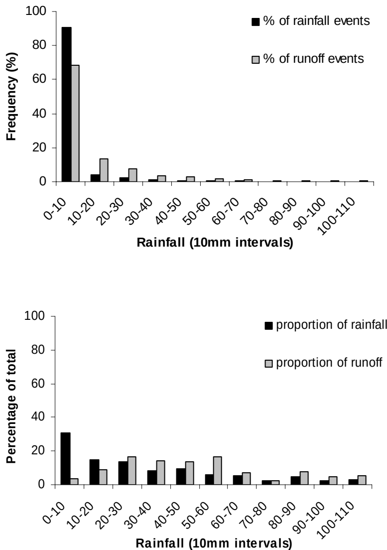
Figure 9.5 (a) Percentage of rainfall and runoff events contributed by each 10mm rainfall event class at the ironbark site (1994–2000). (b). Percentage of the total rainfall received over 6 years and the runoff generated, grouped by 10mm rainfall event class intervals at the ironbark site (1994–2000).
