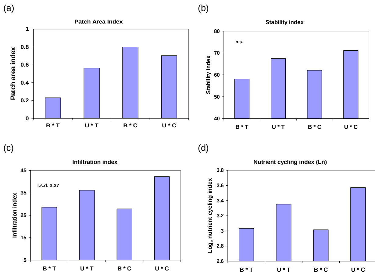
Figure 8.2 Indices of (a) patch areas, (b) stability, (c) infiltration and (d) nutrient cycling, meaned for each burning * tree killing treatment at the poplar box site. B = Burnt, U = Unburnt, T = Treed, C = Treeless.
