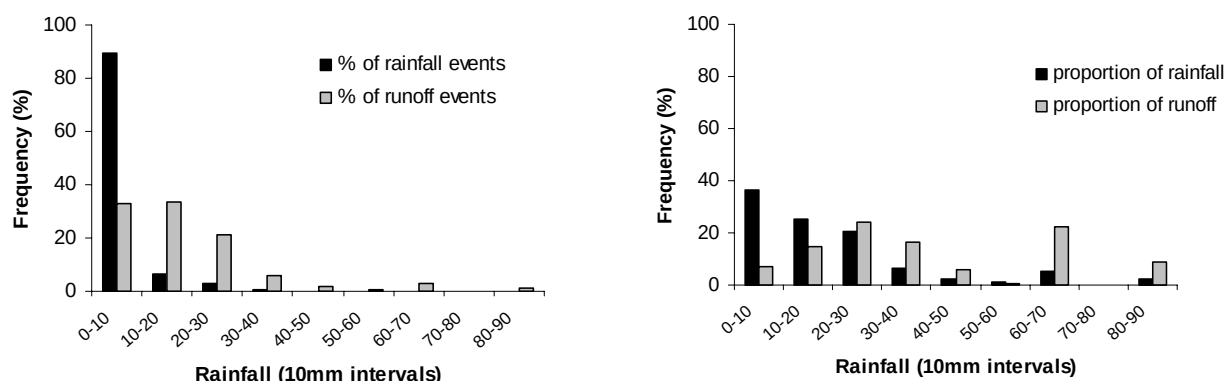
Figure 9.20 (a). Percentage of rainfall and runoff events contributed in each 10mm rainfall event class at the poplar site (1994–2000). (b). Percentage of the total 1994-2000 rainfall and runoff contributed by each 10mm rainfall event class at the poplar box site.
