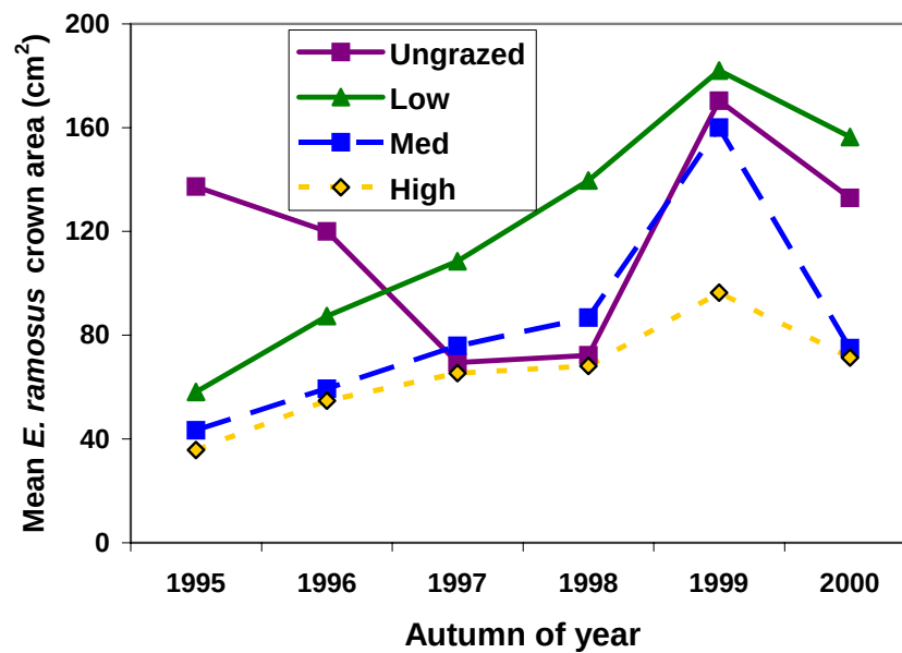
Figure 6.112 Effect of differing grazing pressure on the mean crown area of E. ramosus plants over time.
