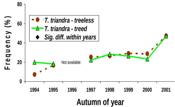
Figure 6.44 Tree killing impact on the frequency of (a) B. ewartiana , (b) C. fallax , (c) H. contortus and (d) T. triandra on ungrazed plots at the ironbark site.
