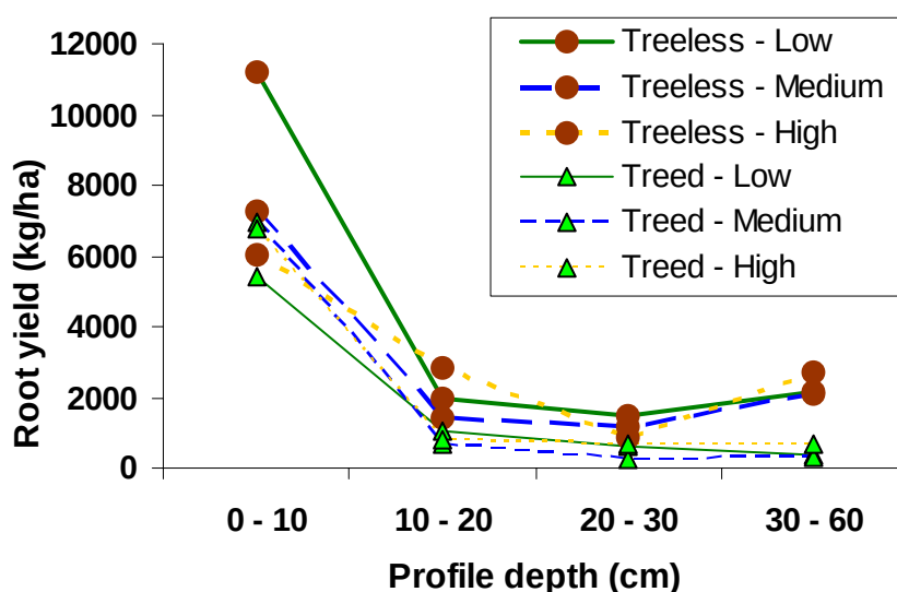
Figure 6.90 Relative grass root dry matter yield in Dec. 2000 at four profile depths for the main grasses in poplar box woodland.
