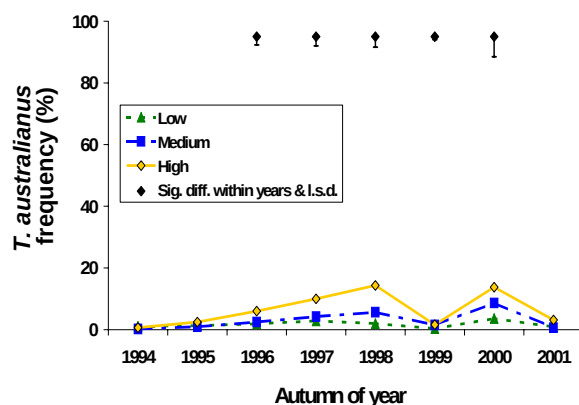
Figure 6.12 Grazing pressure impact on frequency of (a) Aristida spp., (b) Digitaria spp., (c) Enneapogon spp., (d) Native legumes and (e) T. australianus at the ironbark site.
