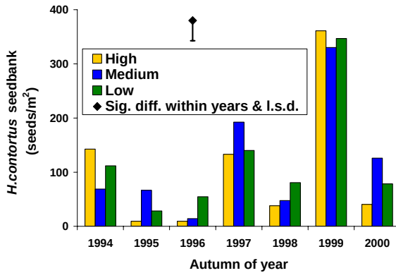
Figure 6.37 Grazing pressure effect over time on the seedbanks of (a) B. ewartiana , (b) C. fallax and (c) H. contortus plants at the ironbark site.
