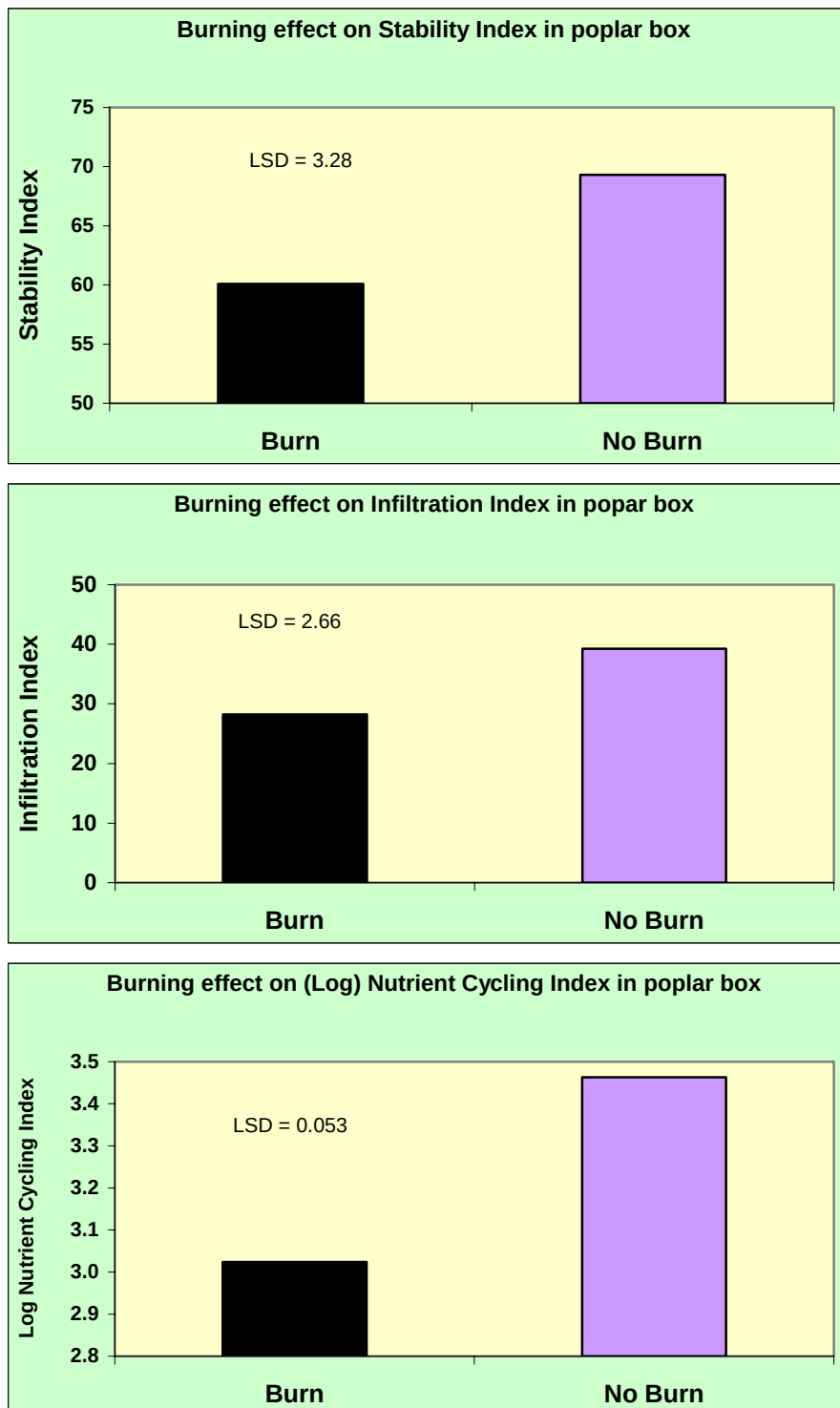
Figures J7 – J9. Histograms showing the effect of regular spring burns on three landscape indices after 7 years without grazing at Glentulloch
