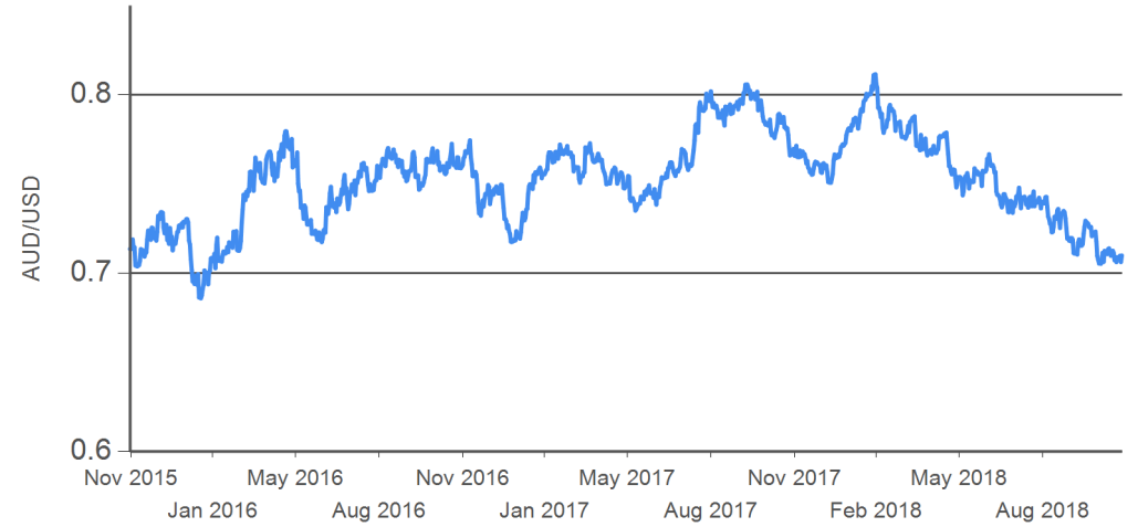
AUD/USD
